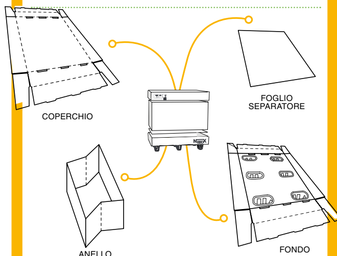
NeboX® Compact
